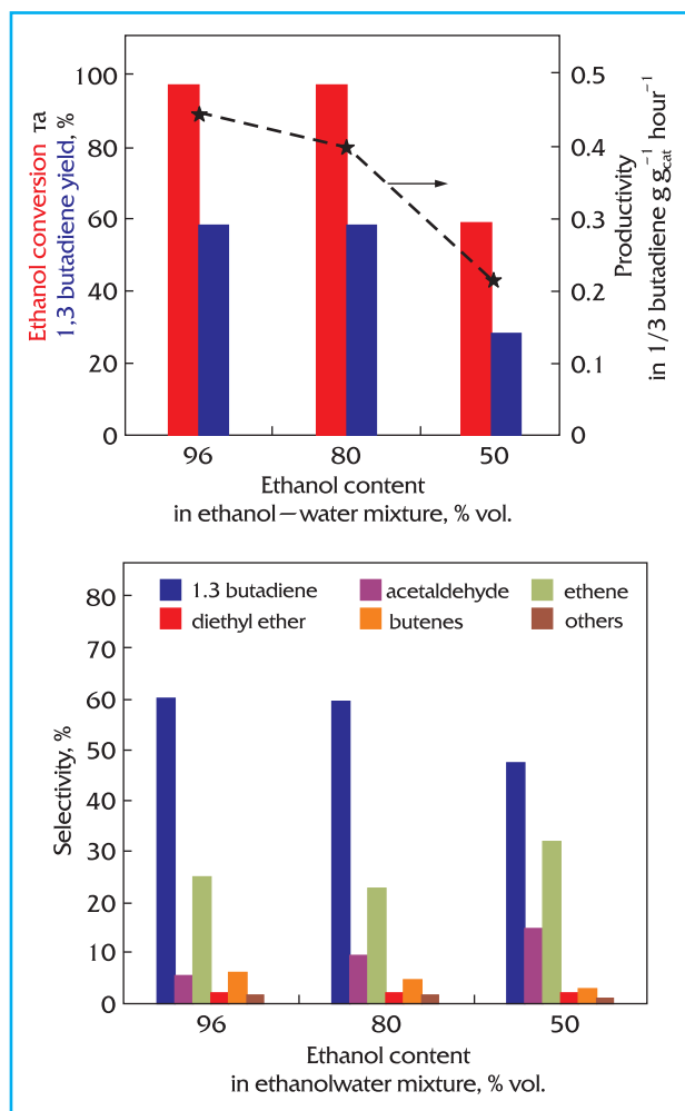
Indicators of the process of transforming ethanol-water mixture into 1,3-butadiene in the presence of ZnO(nano)/ZrO 2 -SiO 2 at the temperature of 400 °C, the load is 1.3 g gc -1 hour -1
