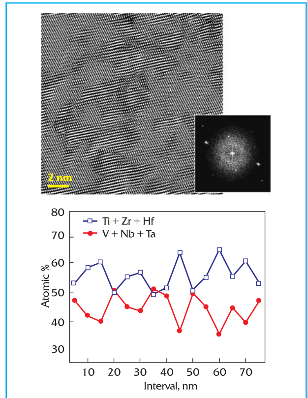
Typical nano-cluster structure of super-hard high-entropy nitride coating, which is due to atom size disparity and nano-level non-uniformity in elements distribution
