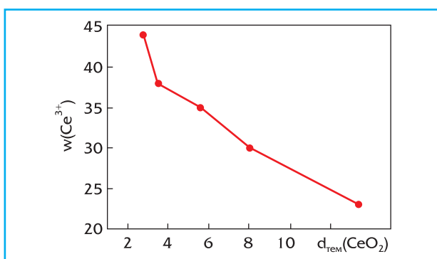
Dependence of \text{Ce}^{3+} ions located on the surfaces of \text{CeO}_2 nanoparticles on their sizes
